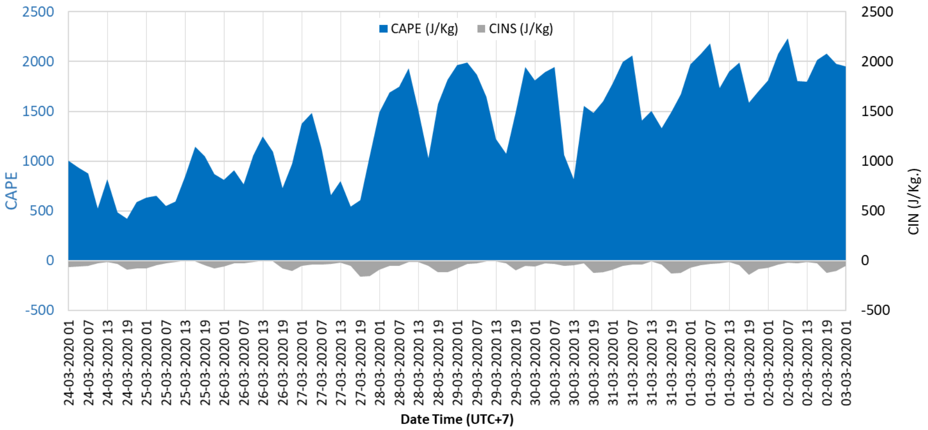
CAPE vs. CINS
