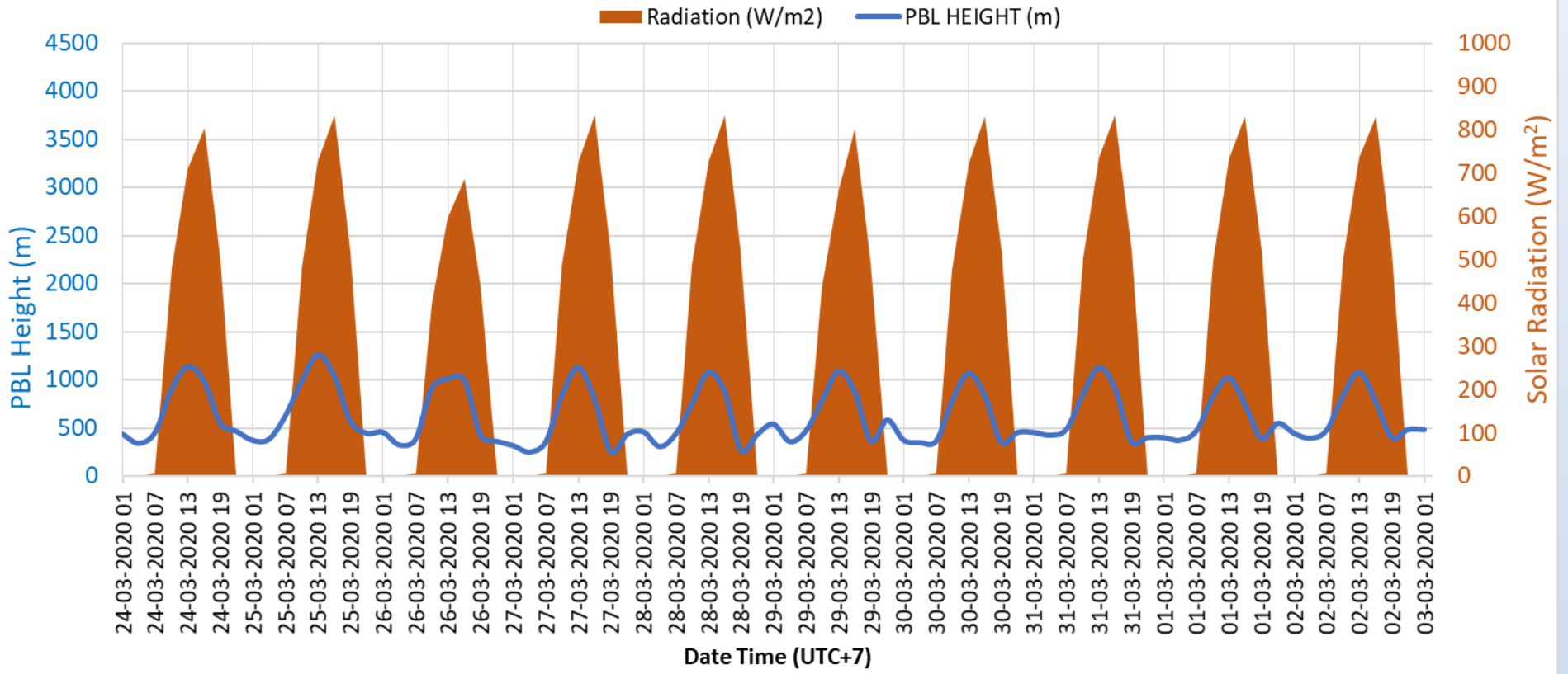
Planetary Boundary Layer Height vs. Solar Radiation
